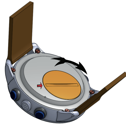
3- Screw the battery cover (4 turns).
